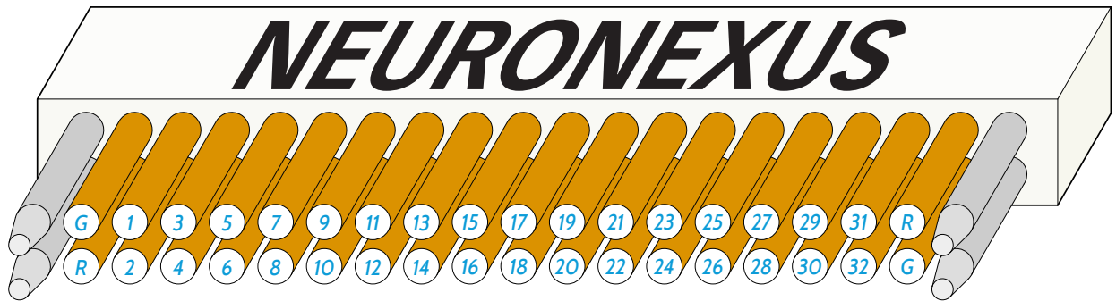
OM32 Connector
